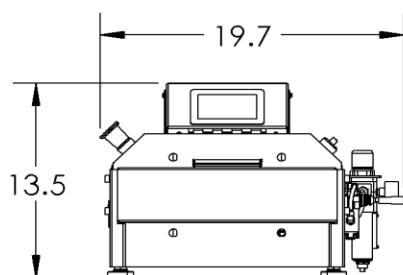
HORIZONTAL ORIENTATION
