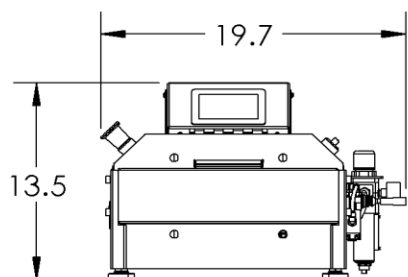
HORIZONTAL ORIENTATION
